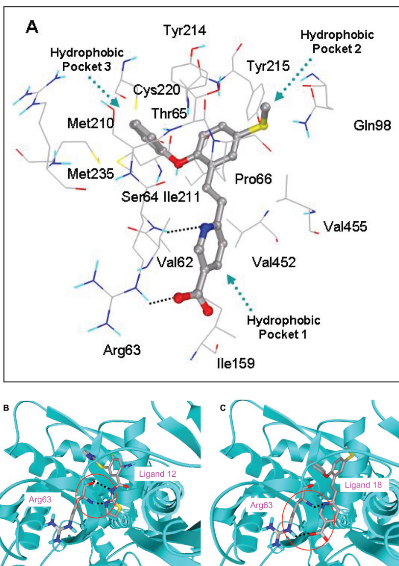
Fig. (10). Binding interactions of ligand 18 (A). Hydrogen bond formation with Arg63 amino acid (B, C).
