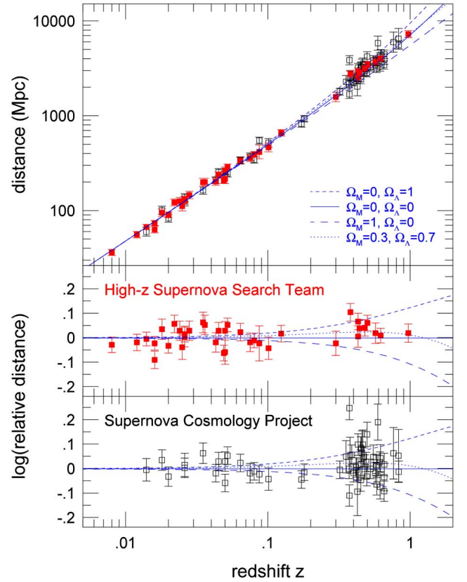
Fig. (1). Shown [10] are the original data points of the High- z Supernova team (filled squares) [1], and the Supernova Cosmology Project (open squares) [2]. The dashed line is the theoretical prediction for a homogeneous and isotropic (FRW) universe which is flat and without cosmological constant ( \Omega_M = 1 , \Omega_\Lambda = 0 ). The solid line is the corresponding prediction for an empty (open) universe ( \Omega_M = 0 , \Omega_\Lambda = 0 ). Also shown (short dashes) is the theoretical prediction for a flat universe with solely a dark energy component ( \Omega_M = 0 , \Omega_\Lambda = 1 ). The dotted line is the solution currently favored for the SN Ia data by both experimental groups ( \Omega_M = 0.3 , \Omega_\Lambda = 0.7 ). For z > 1 , where unfortunately also observational measurements become increasingly difficult, it starts to deviate towards the ( \Omega_M = 1 , \Omega_\Lambda = 0 ) line. The “neo-standard” explanation for this is that \Omega_\Lambda has become dominant only fairly recently ( z \leq 1 ). Observed SN photons within a globally flat universe will always tend towards the line for the open universe, due to inhomogeneous structure formation.
