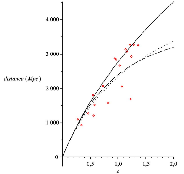
Fig. (2). The prediction of three different homogeneous models are shown together with our simulated inhomogeneous “particles”. The solid line is an open FRW-model with \Omega_M = 0.2 , \Omega_\Lambda = 0 . The dotted line is a flat FRW-model with \Omega_M = 1 , \Omega_\Lambda = 0 . The dashed line is the (flat) Newtonian prediction with corrections for special relativity. An inhomogeneous matter distribution may thus be interpreted wrongly as to suggest that \Omega_M is lower than it actually is, e.g. \Omega_M = 0.2 if interpreted through a homogeneous and isotropic “standard model” cosmology. The simulated particles correspond to \Omega = \Omega_M = 1 . The assumption of homogeneity and isotropy mislead the physical interpretation if the real distribution is inhomogeneous, as is the case for our Universe.
