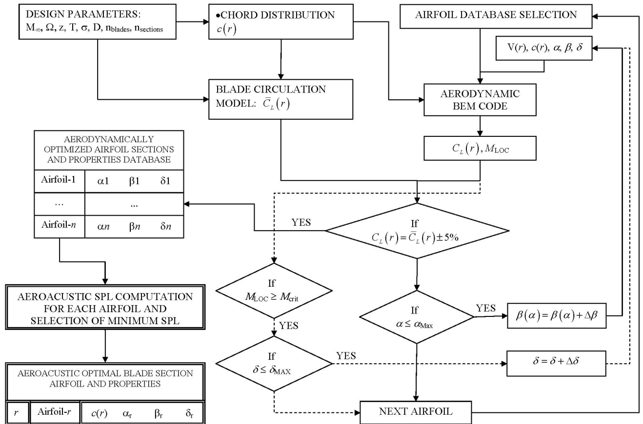
Fig. (1). Aeroacoustic design scheme.
