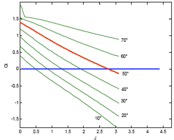
Fig. (6). Thrust coefficient as function of advance ratio and pitch angle at the 75% blade radius. Design configuration in red.
