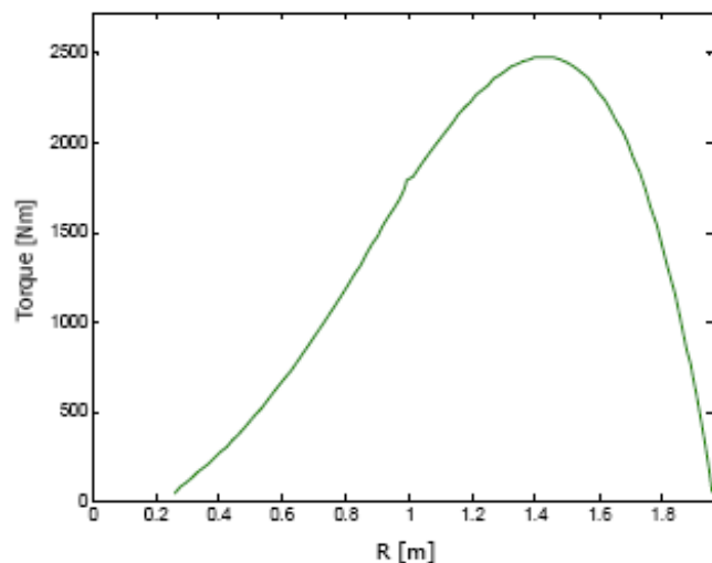
Fig. (5). Torque distribution along the blade radius.
