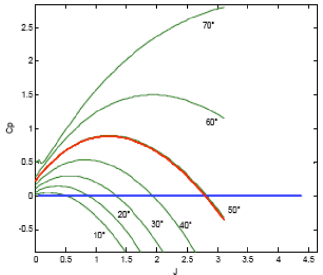
Fig. (7). Power coefficient as function of advance ratio and pitch angle at the 75% blade radius. Design configuration in red.
