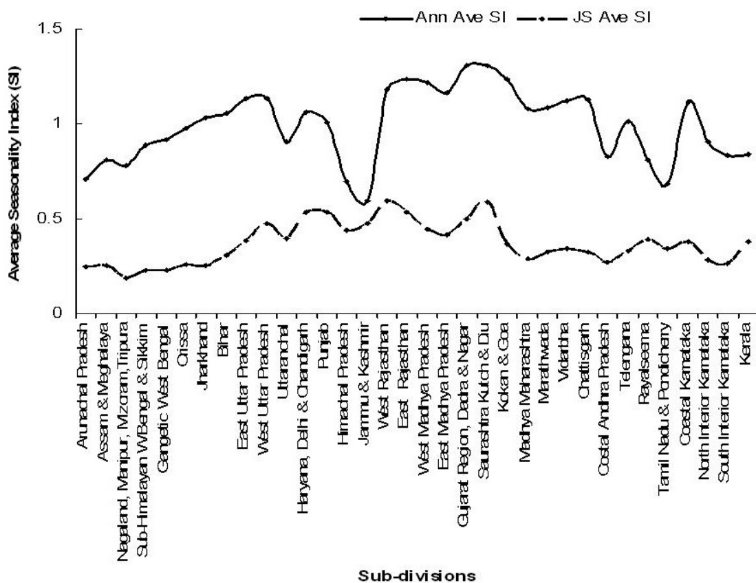
Fig. (5). Average annual and Jun-Sept Seasonality Index (SI) over meteorological sub-divisions.
