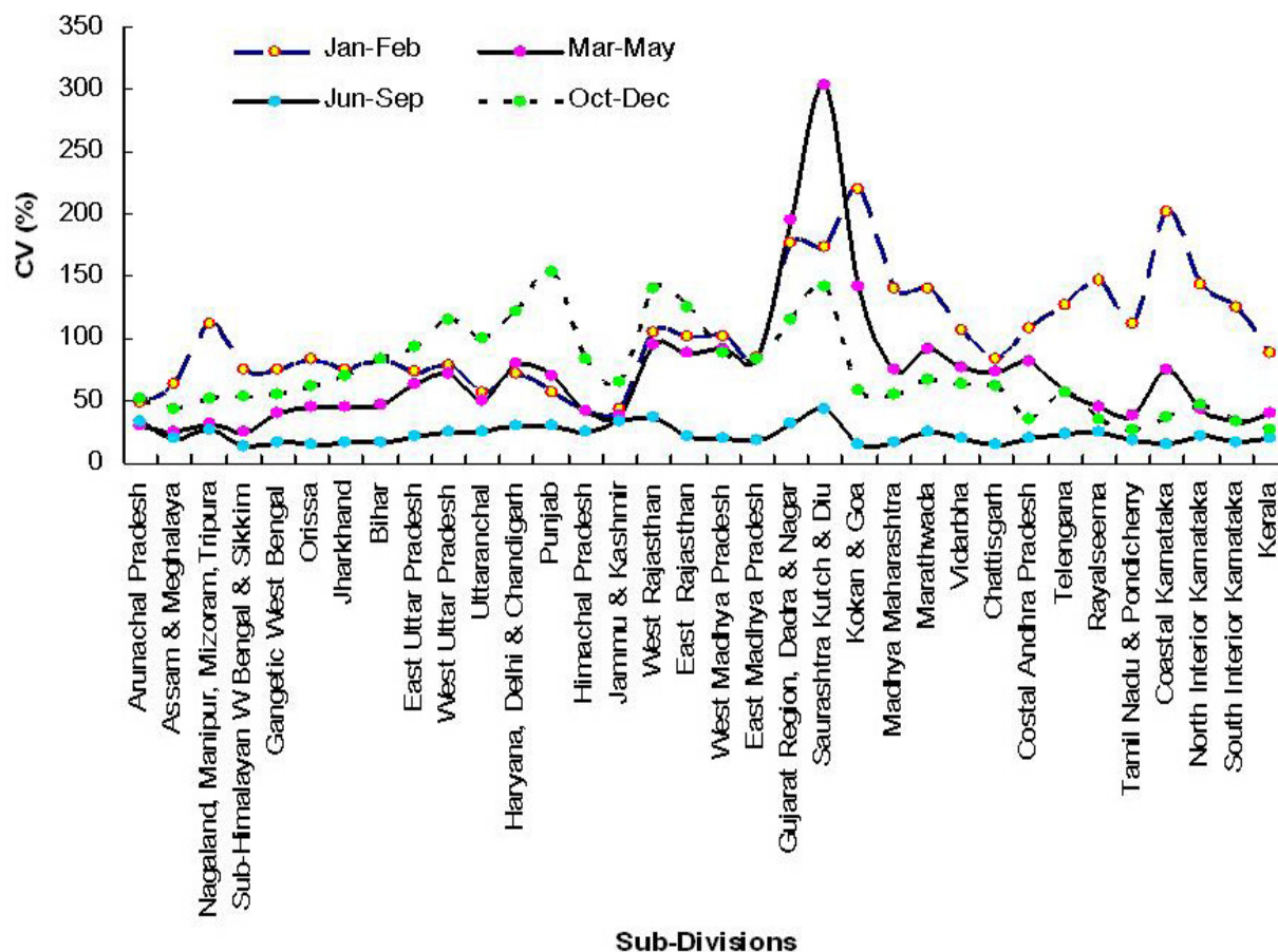
Fig. (3). Variation in CV during winter, pre-monsoon, monsoon and post-monsoon months.
