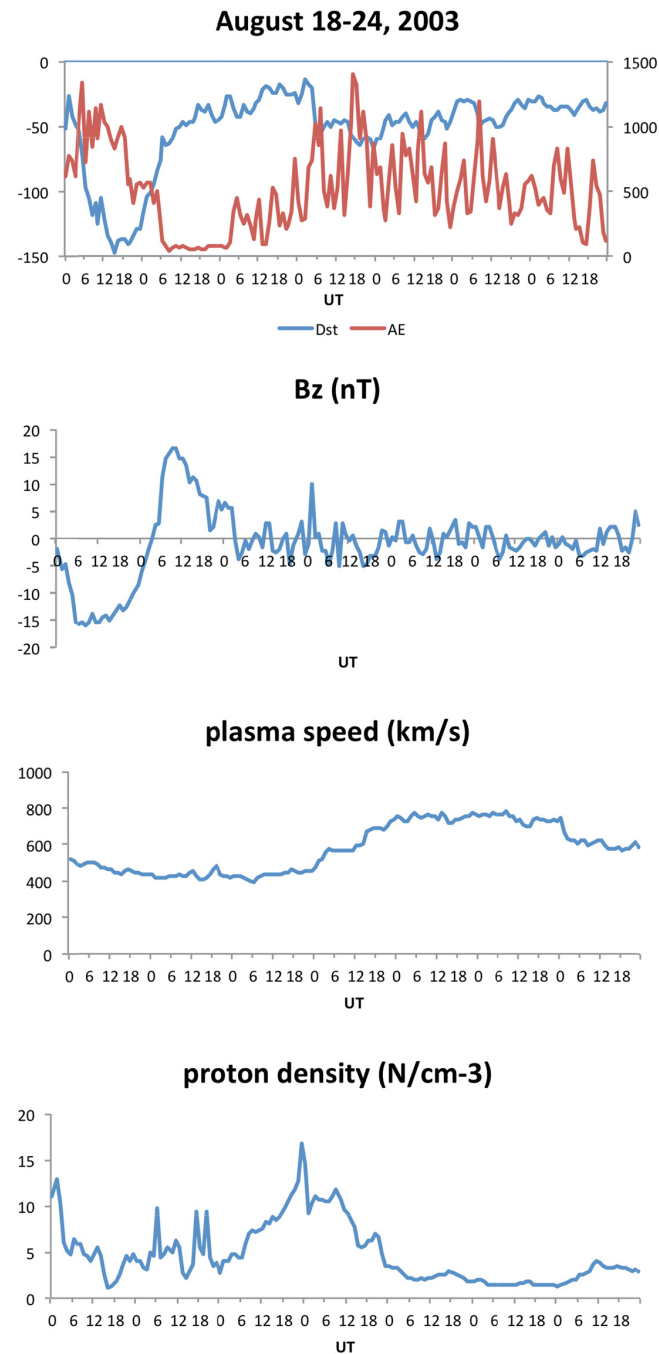
Fig. (5). Geomagnetic/solar activity for the storm period August 18-24, 2003 as indicated by the Dst and AE indexes and the B_z component of the interplanetary magnetic field, the solar wind speed and the proton density, respectively.
