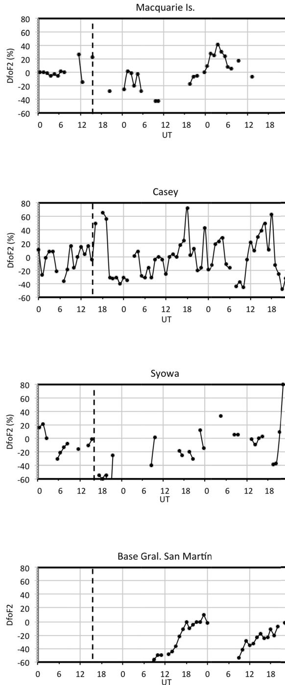
Fig. (4). Ionospheric storm effects observed during October 1-3, 2002 at the stations Macquarie Is., Casey, Syowa and Base Gral. San Martín. The relative deviation of the critical frequency foF2 from the monthly median at each station, DfoF2, is used to describe the perturbations. Dashed line represents the end of the main phase.
