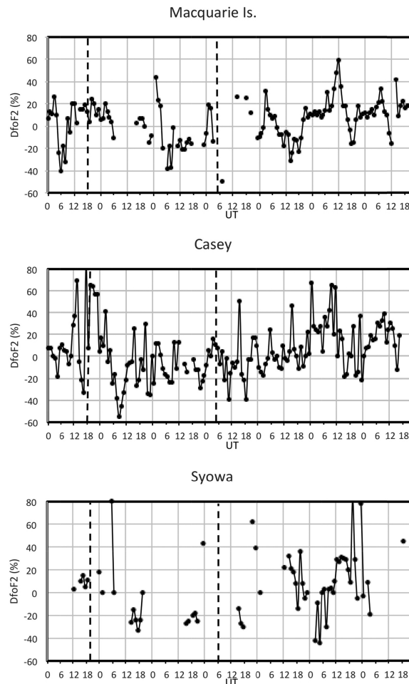
Fig. (2). Ionospheric storm effects observed during August 18-24, 2002 at the stations Macquarie Is., Casey and Syowa. The relative deviation of the critical frequency foF2 from the monthly median at each station, DfoF2, is used to describe the perturbations. Dashed lines indicate the storm onset and the end of the main phase.
