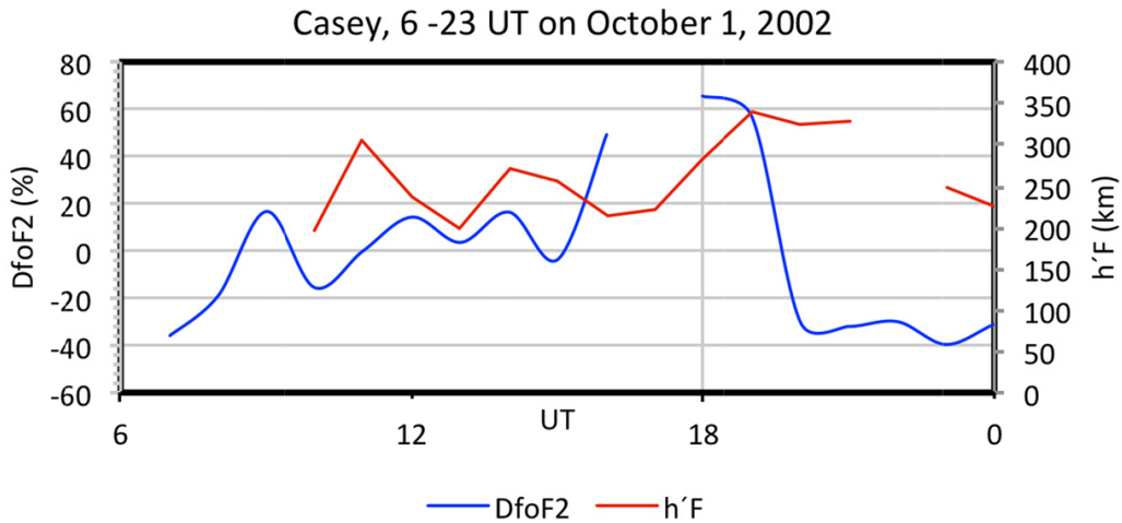
Fig. (7). Temporal variation of DfoF2 and of the virtual height h'F at Casey from 06 to 23 UT on October 1, 2002 (storm 2). Note the uplifting of the F layer and the subsequent increase in foF2 (positive storm).
