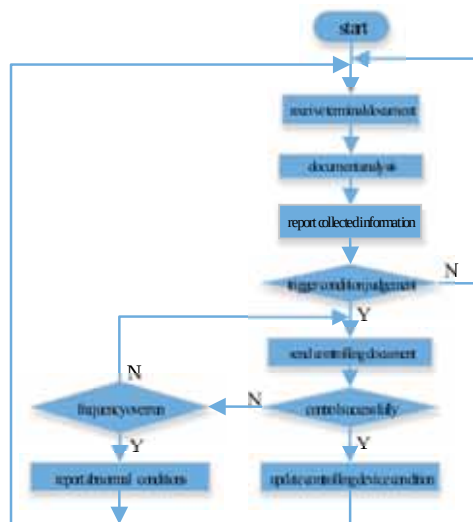
Figure 4 the control procedure with strategy document
