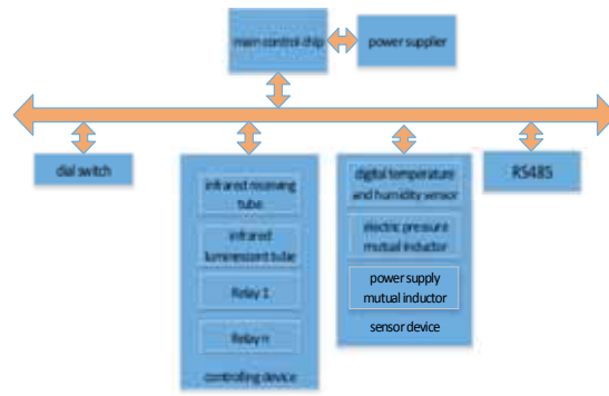
Figure 5 overall structure of terminal
