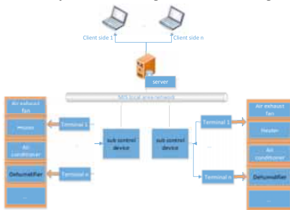
Figure 1: the overall diagram of temperature and humidity monitoring system
