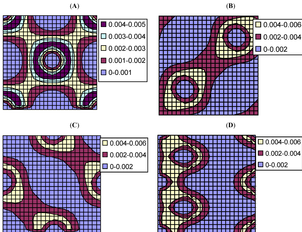
Fig. (2). Valence charge density (in atomic unit) of \alpha – Sn in the: (A) (001) plane, (B) (400) plane, (C) (200) plane, and (D) (110) plane.
