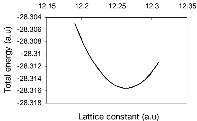
Fig. (1). Total energy of ( \alpha - \text{Sn} ) as a function of lattice constant.
