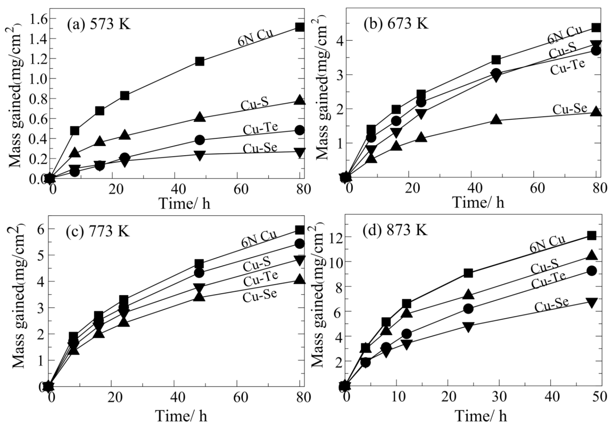
Fig. (1). Mass gain as a function of time for samples oxidized at 573-873 K in 0.1 MPa O 2 . (a) 573 K, 80 h; (b) 673 K, 80 h; (c) 773 K, 80 h; (d) 873 K, 48 h.
