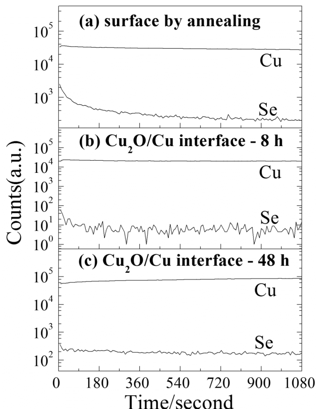
Fig. (3). SIMS depth profiles of Cu and Se for Cu-Se alloys sputtered from (a) surface after annealing; (b) \text{Cu}_2\text{O}/\text{Cu} interface oxidized at 773 K for 8 h; (c) \text{Cu}_2\text{O}/\text{Cu} interface oxidized at 773 K for 48 h.
