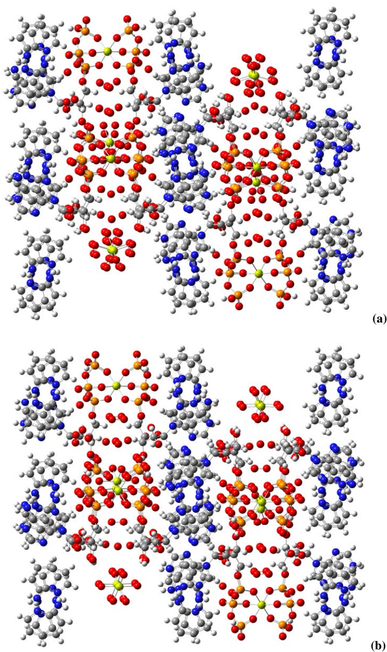
Fig. (1). Packing diagrams for [\text{Mg}(\text{H}_2\text{O})_6][\text{Mg}(\text{HATP})_2]\cdot 2(\text{HDPA})\cdot x\text{H}_2\text{O} 1 as viewed almost along cell axis a for: (a) x = 12 , data set DS2; (b) x = 6 , DS3. It has to be noted that the [\text{Mg}(\text{H}_2\text{O})_6]^{2+} cation is disordered in (a) but not in (b). The occupancy for the free water molecule oxygen atoms for (b) is 1 (O2WD), 0.5 (O1WD, oxygen on special position), 0.25 (O3WD, O4WD), and 0.5 (O5WD, O6WD); whereas the occupancy for the corresponding water molecule oxygen atoms in (a) are 1, 0.5, 1, 1 (as regard naming of atoms and occupancy value, see the respective CIF files, supplementary material).
