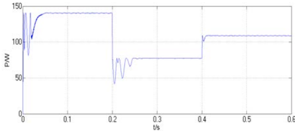
(a) P_{out} by the method of PID
