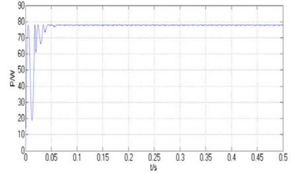
(a) P_{out} by the method of PID
