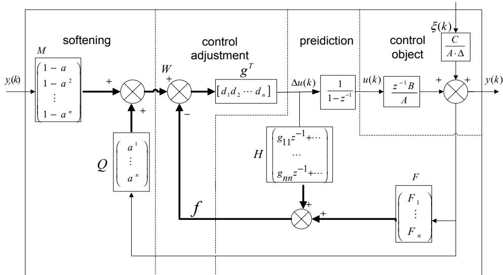
Fig. 4 GPC algorithm structure
