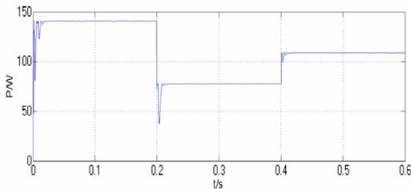
(a) P_{out} by the method of PID
