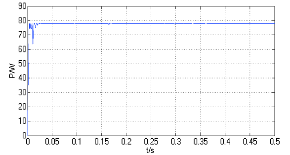
(b) P_{out} by the method of GPC
