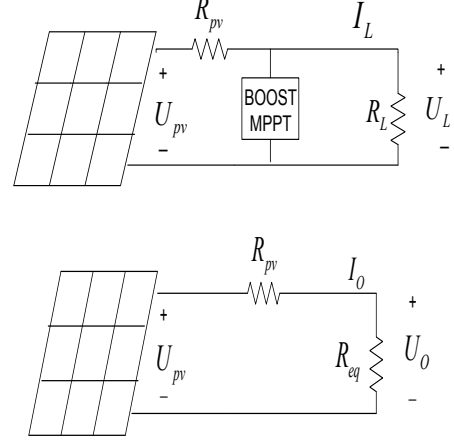
Fig. 2 Equivalent transformation of Boost circuit
