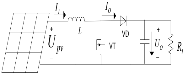
Fig. 1 Boost schematic diagram
