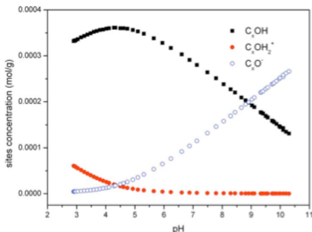
Fig. (2B). Distribution of surface site concentrations of MWCNTs ( 5.0\text{ g/L} ) as a function of pH at I=0.01\text{M NaClO}_4 and T=20^\circ\text{C} .
