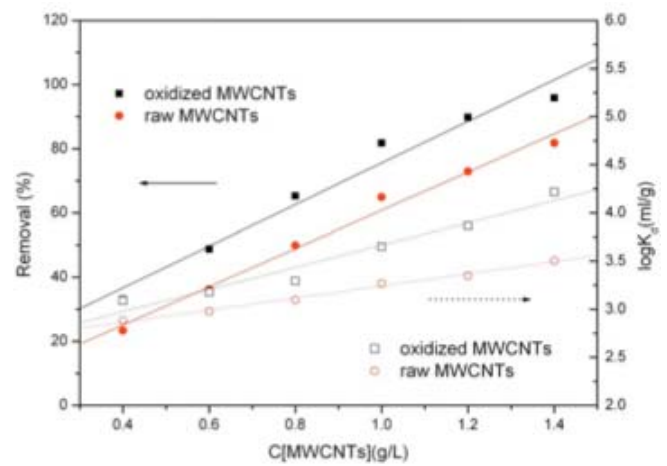
Fig. (7). Removal of Cr(VI) on the oxidized and raw MWCNTs as a function of MWCNT content. C[\text{Cr(VI)}]_{\text{initial}}=3.0 \text{ mg/L} , I=0.01 \text{ M NaClO}_4 , T=20\pm 1^\circ\text{C} , contact time=165 h, \text{pH}=2.88\pm 0.02 .
