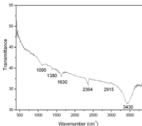
Fig. (1B). FTIR spectrum of raw MWCNT sample.
