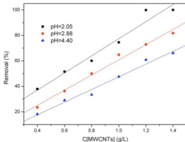
Fig. (3). Removal of Cr(VI) as a function of raw MWCNT content at different pH values. C[\text{Cr(VI)}]_{\text{initial}}=3.0\text{ mg/L} , I=0.01\text{M NaClO}_4 , T=20\pm 1^\circ\text{C} , contact time=165 h.
