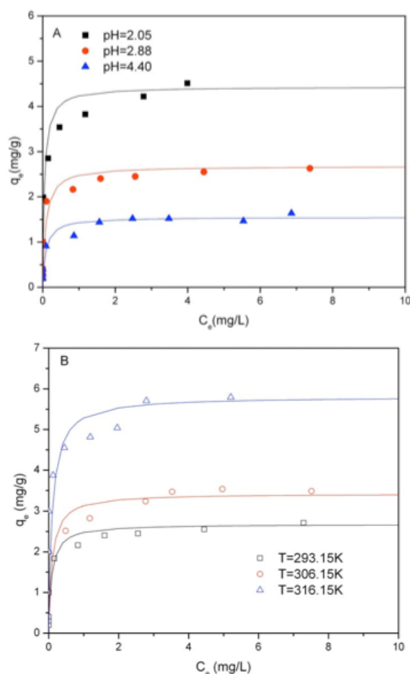
Fig. (4). Adsorption isotherms of Cr(VI) on raw MWCNTs. I=0.01\text{M NaClO}_4 , m/V=1.0\text{ g/L} , and contact time=165 h. (A): at different pH values at T=20\pm10\text{ }^\circ\text{C} ; (B): at different temperatures at \text{pH}=2.88\pm0.02 .
