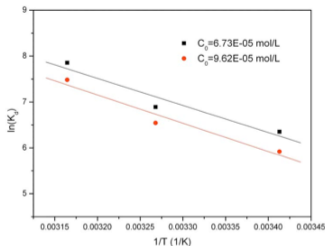
Fig. (8). Plot of distribution coefficient K_d vs. temperature for Cr(VI) adsorption on the raw MWCNTs. I=0.01M NaClO 4 , m/V=1.0 g/L, pH=2.88±0.02.
